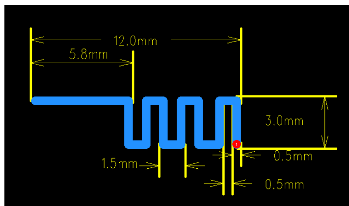
Figure 1 :Keyboard Antenna size
