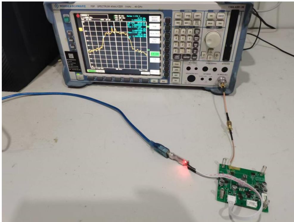
RF test Setup:
