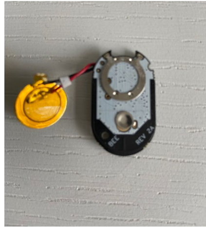
Bottom of Tag PCB and piezo
