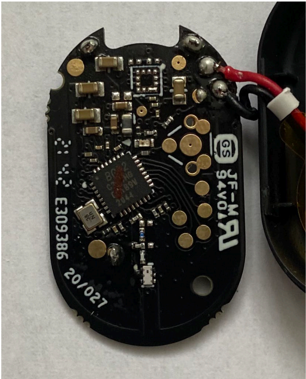
Top side of PCB
