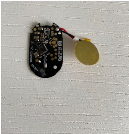
Top of Tag PCB and piezo
