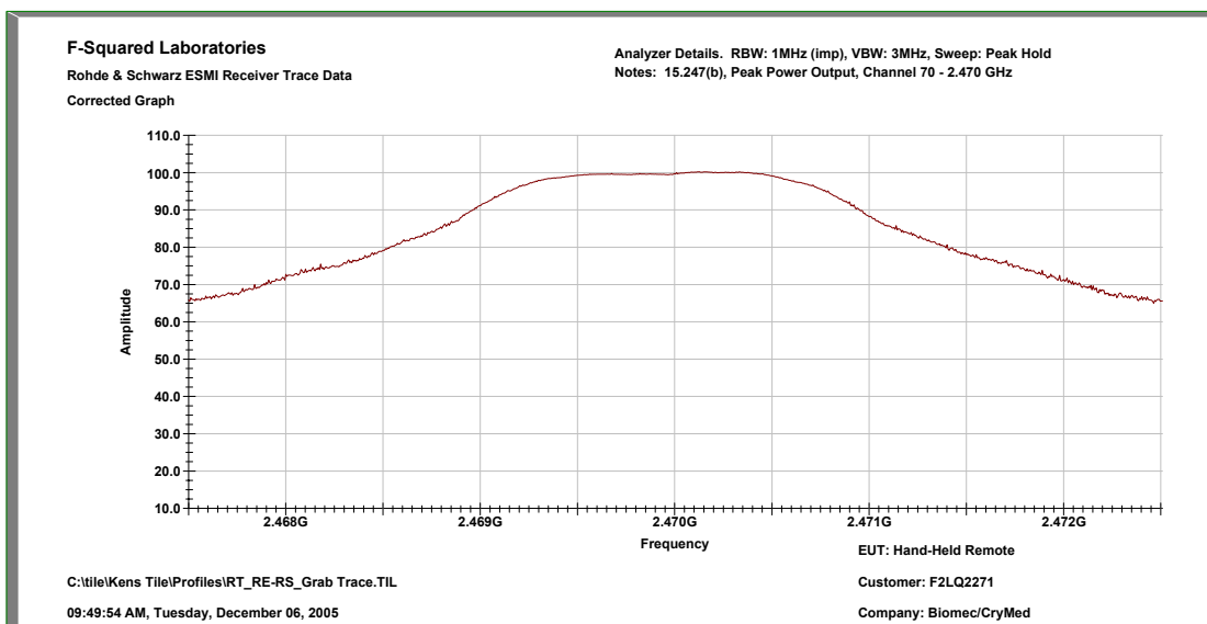
Figure 6: Peak Power Output, Upper Channel
