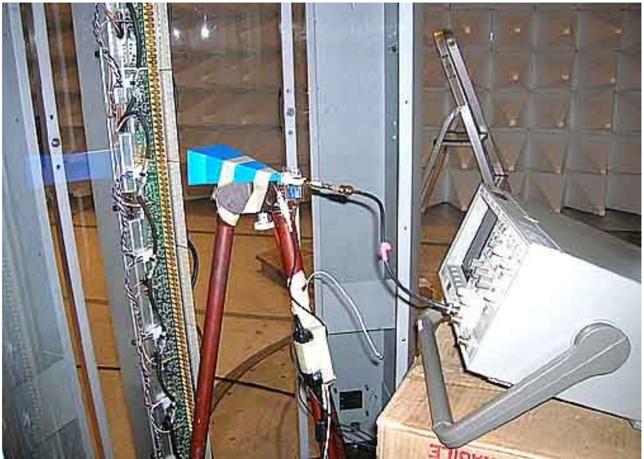
PHOTOGRAPH SHOWING DUTY CYCLE MEASUREMENT SETUP
