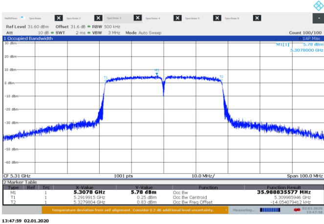
Figure 8.6-2: 99 % bandwidth on 40 MHz, sample plot
