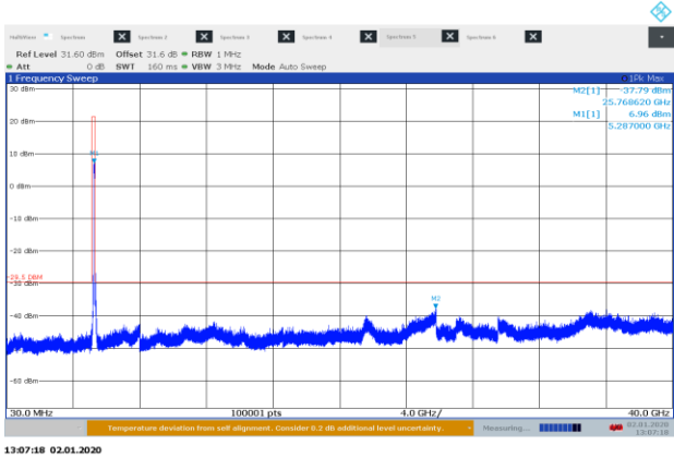
Figure 8.8-53: Conducted spurious emissions 30 MHz – 40 GHz low channel, 802.11ac ch0
