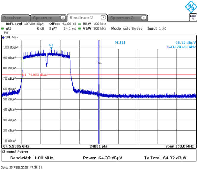
Figure 8.8-5: Peak spurious emissions within restricted bands at high channel, 802.11n cho
