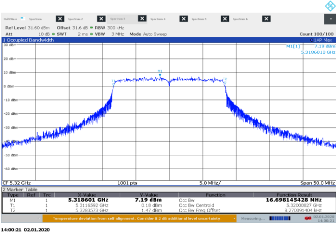
Figure 8.6-1: 99 % bandwidth on 20 MHz, sample plot
