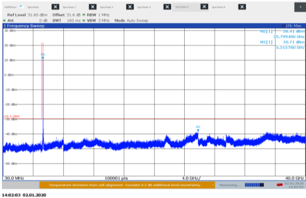
Figure 8.8-47: Conducted spurious emissions 30 MHz – 40 GHz high channel, 802.11a ch 0
