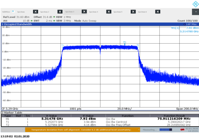
Figure 8.6-3: 99 % bandwidth on 80 MHz, sample plot
