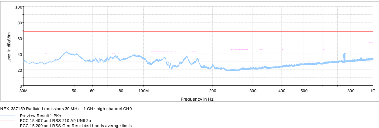
Figure 8.8-15: Radiated spurious emissions 30 MHz – 1 GHz high channel cho
