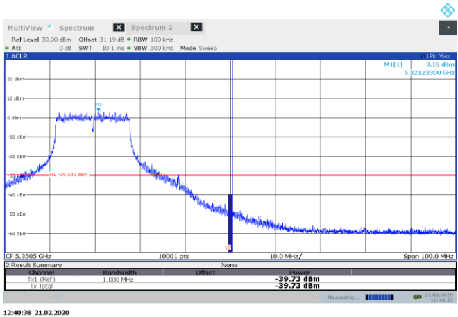
Figure 8.8-34: Conducted emissions at band edge measurement, channel 64, 802.11a ch1
