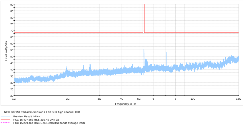
Figure 8.8-24: Radiated spurious emissions 1 - 18 GHz high channel, ch1
