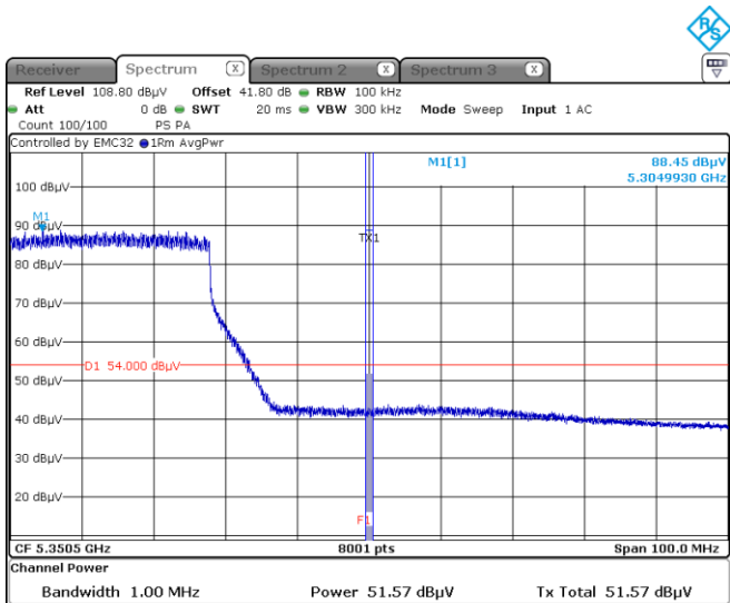
Figure 8.8-10: Average spurious emissions within restricted bands at high channel, 802.11ac cho
