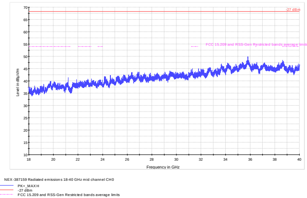
Figure 8.8-26: Radiated spurious emissions 18 - 40 GHz mid channel, cho
