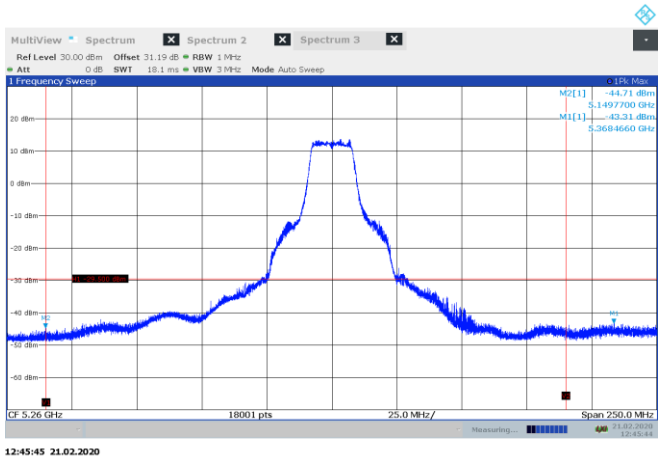
Figure 8.8-32: Conducted emissions at band edge measurement, channel 52, 802.11a ch1
