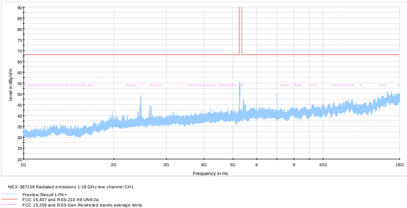
Figure 8.8-22: Radiated spurious emissions 1 - 18 GHz low channel, ch1
