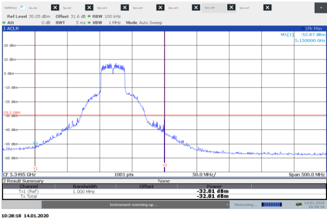
Figure 8.8-36: Conducted emissions at band edge measurement, channel 54, 802.11n ch1
