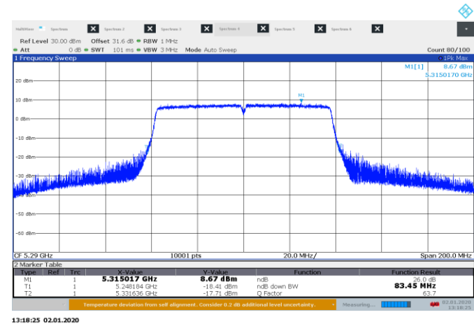
Figure 8.5-3: 26 dB bandwidth on 80 MHz, sample plot
