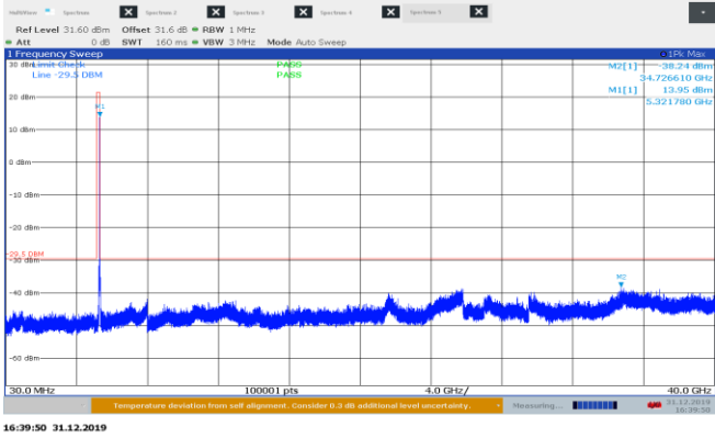
Figure 8.8-48: Conducted spurious emissions 30 MHz – 40 GHz high channel, 802.11a ch 1
