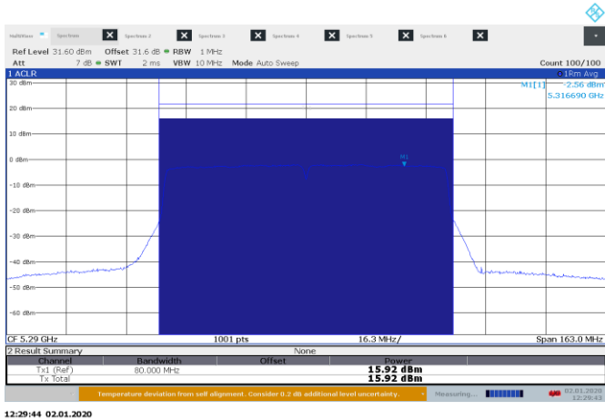
Figure 8.7-3 : Sample plot for power and PSD on 802.11ac
