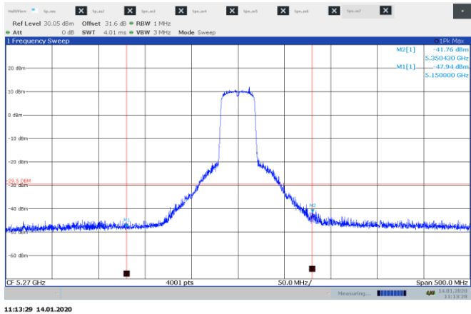
Figure 8.8-35: Conducted emissions at band edge measurement, channel 54, 802.11n cho
