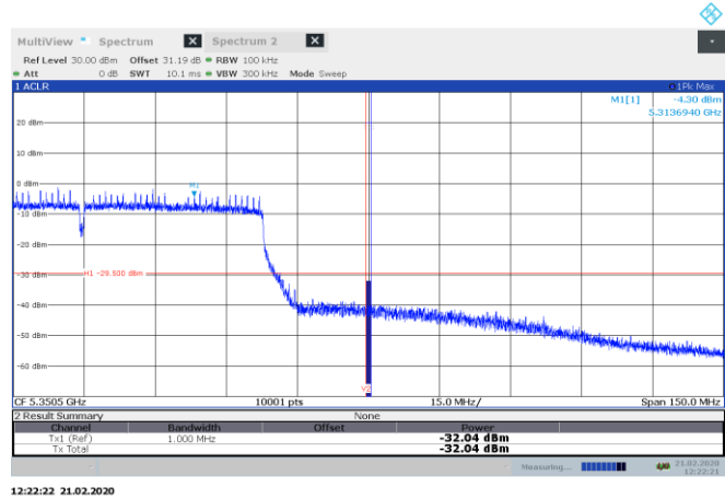
Figure 8.8-40: Conducted emissions at band edge measurement, channel 54, 802.11ac ch1
