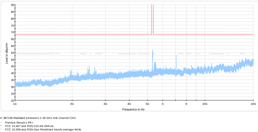
Figure 8.8-23: Radiated spurious emissions 1 - 18 GHz mid channel, ch1
