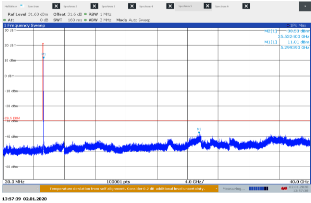
Figure 8.8-45: Conducted spurious emissions 30 MHz – 40 GHz mid channel, 802.11a ch 0
