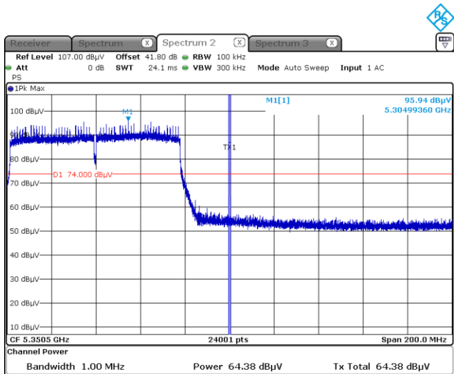
Figure 8.8-9: Peak spurious emissions within restricted bands at high channel, 802.11ac cho
