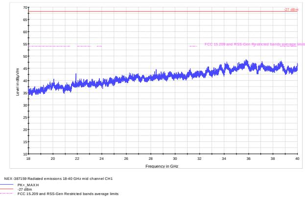
Figure 8.8-29: Radiated spurious emissions 18 - 40 GHz mid channel, ch1
