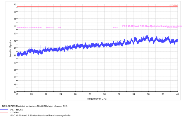
Figure 8.8-30: Radiated spurious emissions 18 - 40 GHz high channel, ch1
