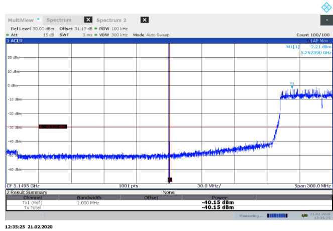
Figure 8.8-42: Conducted emissions at band edge measurement, channel 54, 802.11ac ch1 lower band edge
