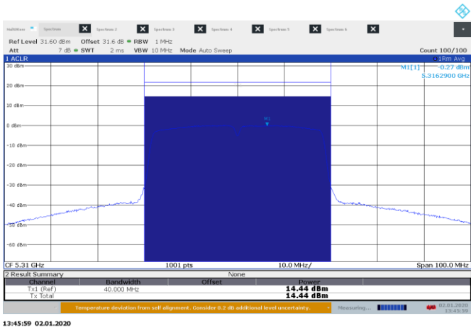
Figure 8.7-2: Sample plot for power and PSD on 802.11n
