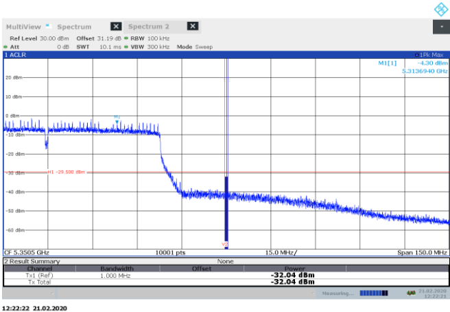
Figure 8.8-38: Conducted emissions at band edge measurement, channel 62, 802.11n ch1
