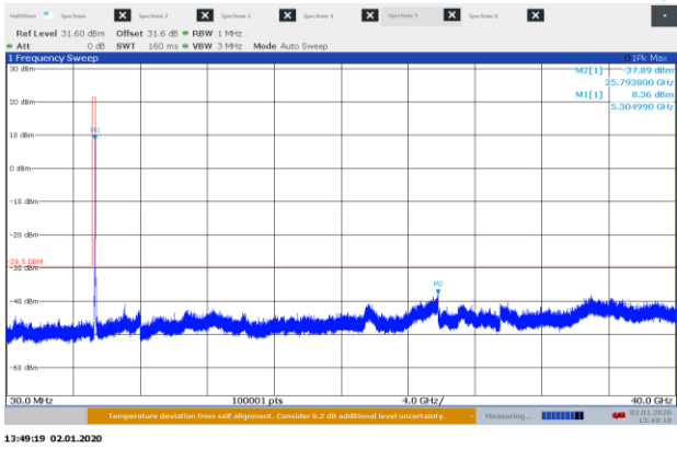
Figure 8.8-51: Conducted spurious emissions 30 MHz – 40 GHz high channel, 802.11n ch0
