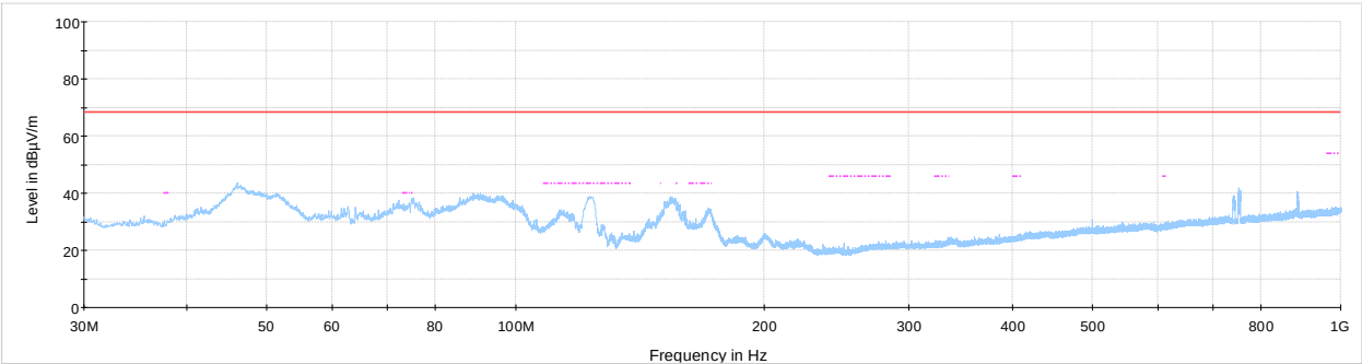
NEX-387159 Radiated emissions 30 MHz - 1 GHz mid channel CH1 Preview Result 1-PK+ FCC 15.407 and RSS-210 A9 UNII-2a FCC 15.209 and RSS-Gen Restricted bands average limits
