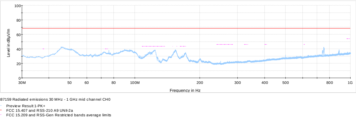
Figure 8.8-14: Radiated spurious emissions 30 MHz – 1 GHz mid channel cho
