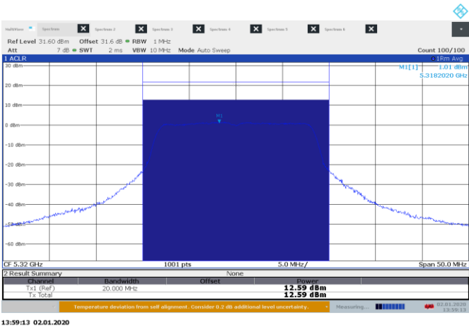
Figure 8.7-1: Sample plot for power and PSD on 802.11a
