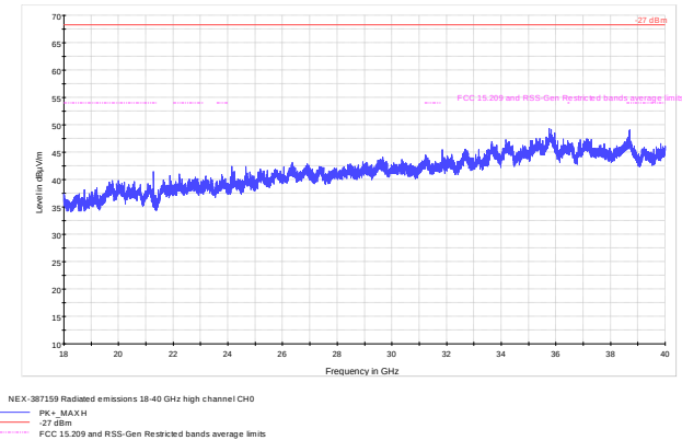
Figure 8.8-27: Radiated spurious emissions 18 - 40 GHz high channel, cho
