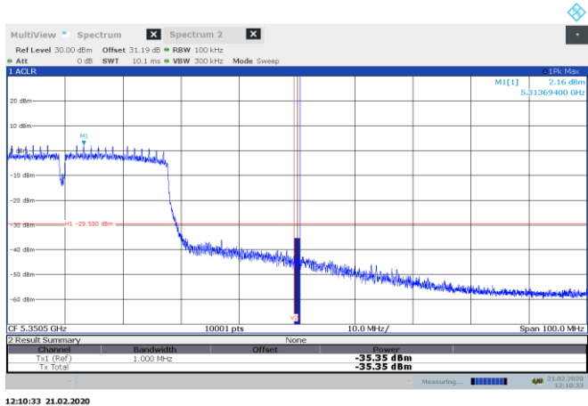
Figure 8.8-37: Conducted emissions at band edge measurement, channel 62, 802.11n cho
