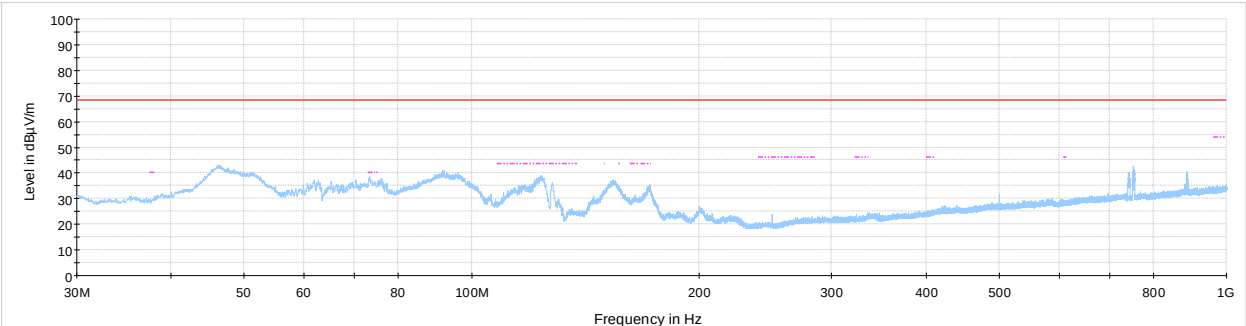
NEX-387159 Radiated emissions 30 MHz - 1 GHz low channel CH1 Preview Result 1-PK+ FCC 15.407 and RSS-210 A9 UNII-2a FCC 15.209 and RSS-Gen Restricted bands average limits
