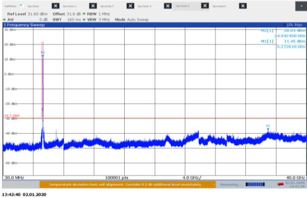
Figure 8.8-43: Conducted spurious emissions 30 MHz – 40 GHz low channel, 802.11a ch 0
