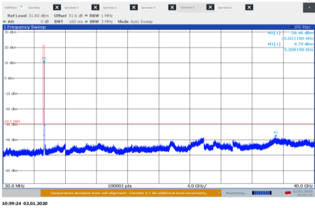
Figure 8.8-49: Conducted spurious emissions 30 MHz – 40 GHz low channel, 802.11n ch0
