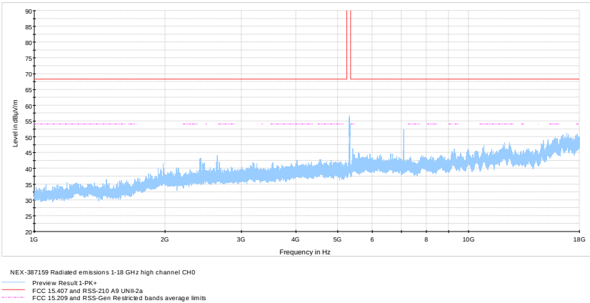
Figure 8.8-21: Radiated spurious emissions 1 - 18 GHz high channel, cho
