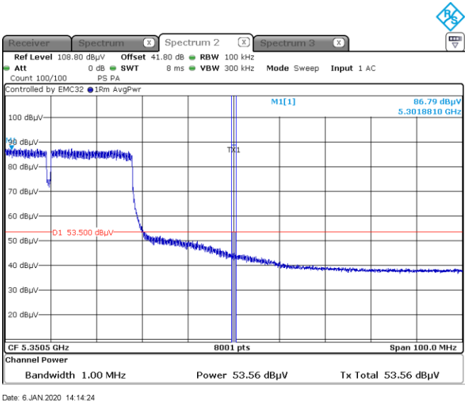
Figure 8.8-6: Average spurious emissions within restricted bands at high channel, 802.11n cho
