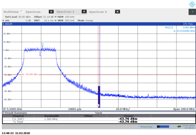
Figure 8.8-33: Conducted emissions at band edge measurement, channel 64, 802.11a ch0
