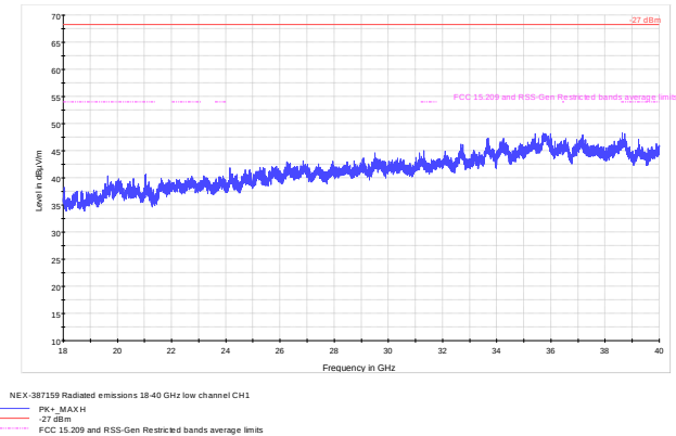
Figure 8.8-28: Radiated spurious emissions 18 - 40 GHz low channel, ch1
