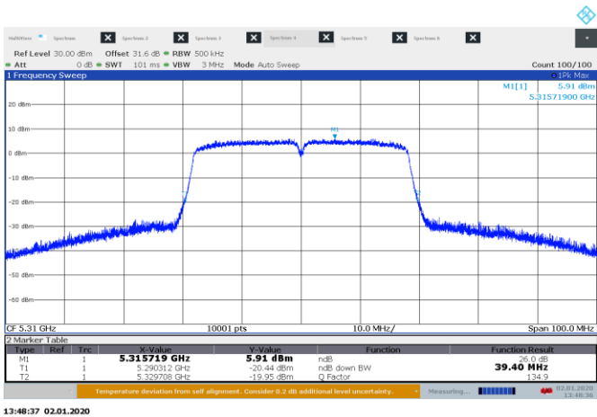
Figure 8.5-2: 26 dB bandwidth on 40 MHz, sample plot
