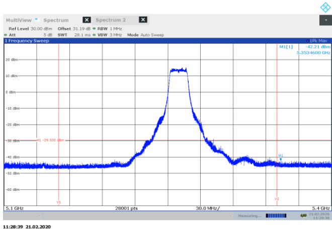
Figure 8.8-31: Conducted emissions at band edge measurement, channel 52, 802.11a ch0
