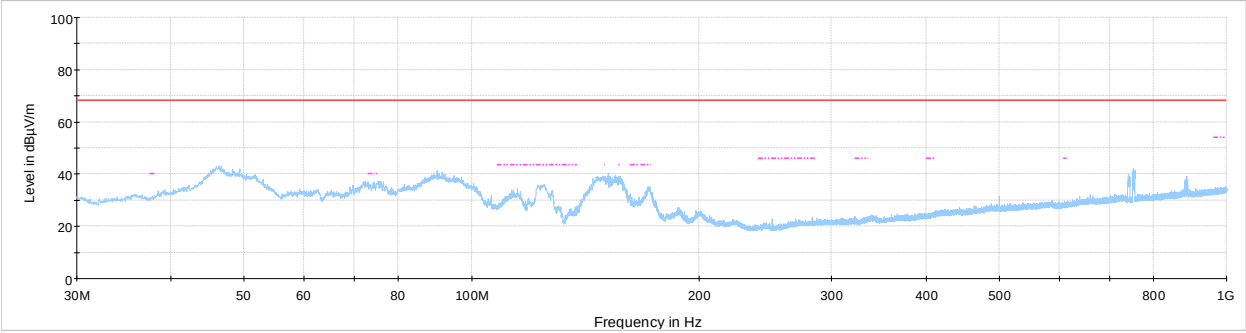
NEX-387159 Radiated emissions 30 MHz - 1 GHz high channel CH1 Preview Result 1-PK+ FCC 15.407 and RSS-210 A9 UNII-2a FCC 15.209 and RSS-Gen Restricted bands average limits
