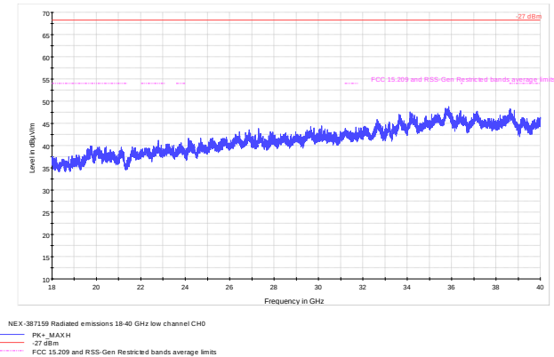
Figure 8.8-25: Radiated spurious emissions 18 - 40 GHz low channel, cho
