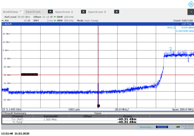
Figure 8.8-41: Conducted emissions at band edge measurement, channel 54, 802.11ac cho lower band edge
