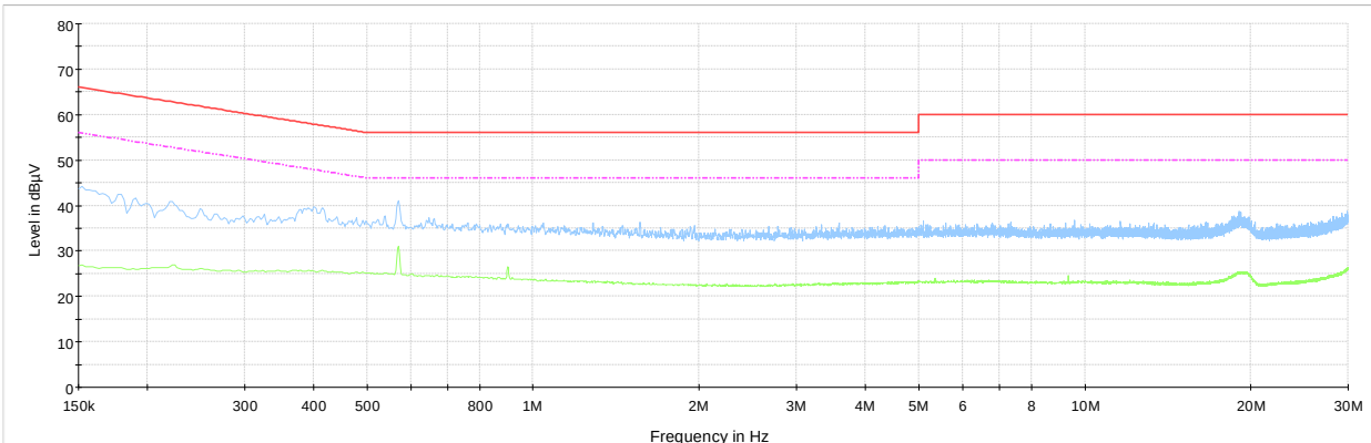
Figure 8.4-1: AC power line conducted emissions – spectral plot on phase line
