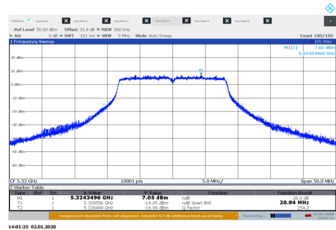
Figure 8.5-1: 26 dB bandwidth on 20 MHz, sample plot
