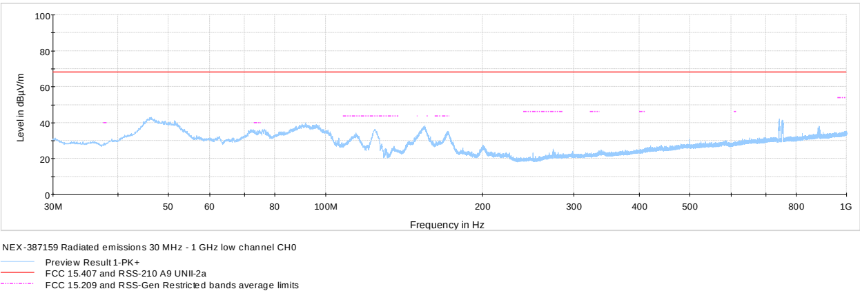
Figure 8.8-13: Radiated spurious emissions 30 MHz – 1 GHz low channel cho
