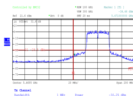
Figure 8.8-38: Conducted band edge emissions 5.47 GHz, channel 102, 802.11n ch1
