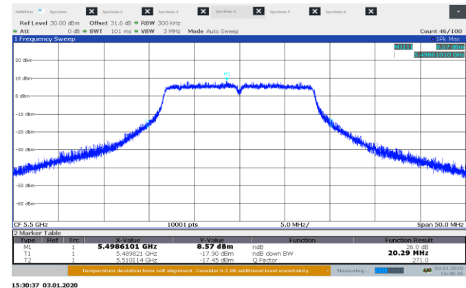
Figure 8.5-1: 26 dB bandwidth on 802.11a, sample plot
