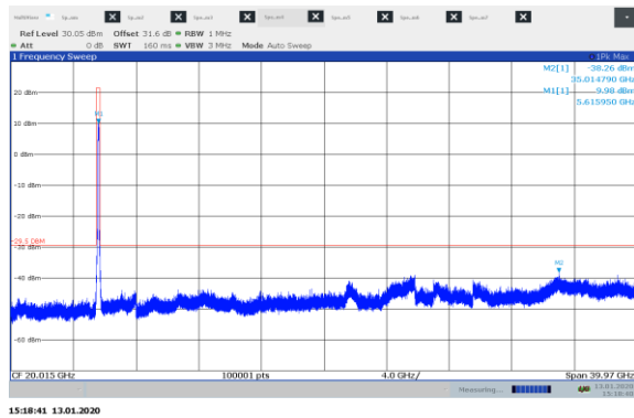
Figure 8.8-63: Conducted spurious emissions 30 MHz – 40 GHz mid channel, 802.11ac ch0
