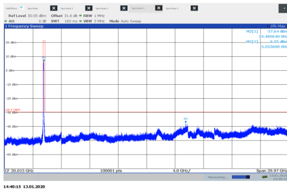
Figure 8.8-61: Conducted spurious emissions 30 MHz – 40 GHz low channel, 802.11ac ch0
