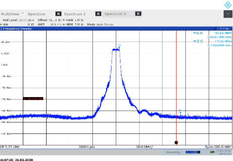
Figure 8.8-35: Conducted band edge emissions 5.85 GHz, channel 144, 802.11a cho
