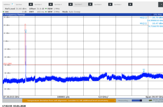
Figure 8-59: Conducted spurious emissions 30 MHz – 40 GHz high channel, 802.11n cho
