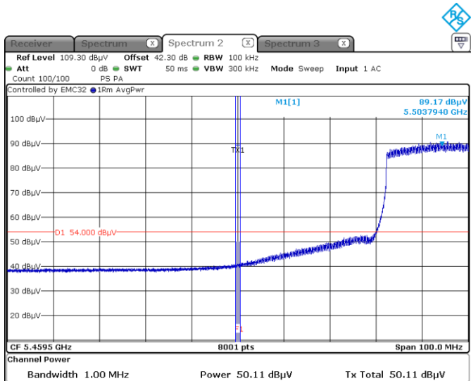
Figure 8.8-6: Average spurious emissions within restricted bands at 5.46 GHz, low channel, 802.11n ch0
