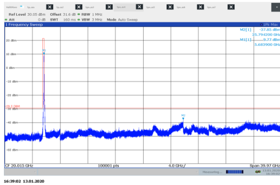
Figure 8.8-65: Conducted spurious emissions 30 MHz – 40 GHz high channel, 802.11ac ch0
