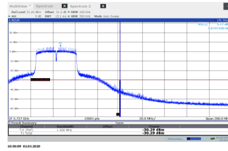
Figure 8.8-40: Conducted band edge emissions 5.725 GHz, channel 134, 802.11n ch1
