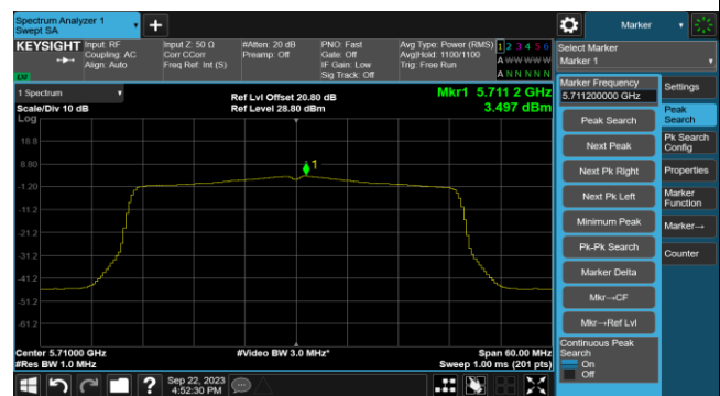
Channel 142(5710MHz)
