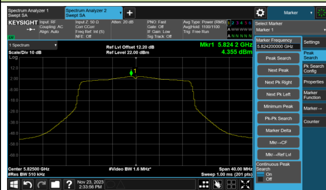
Channel 165 (5825MHz)
