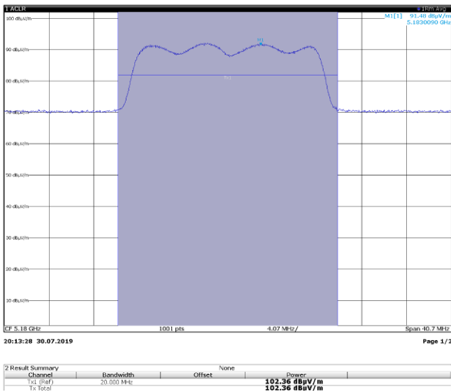
PSD on 802.11nHT20 Sample plot, vertical
