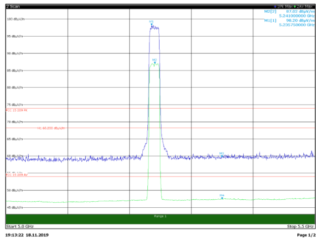
Band edge bands, Tx on 5240 MHz, 802.11a vertical
