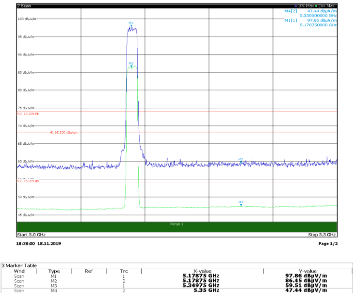
Band edge bands, Tx on 5180 MHz, 802.11 Nht20 horizontal
