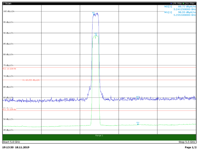
Band edge bands, Tx on 5240 MHz, 802.11a horizontal
