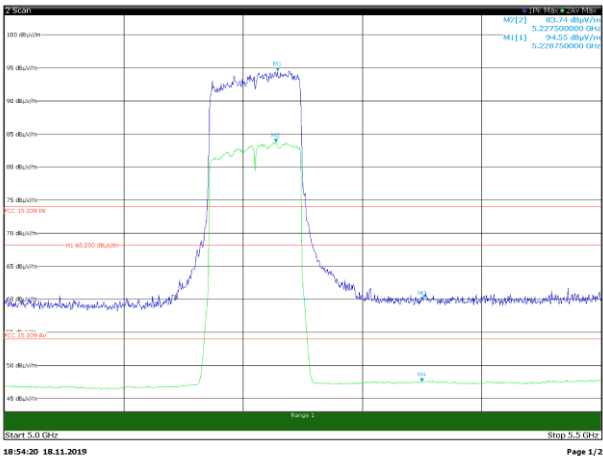
Band edge bands, Tx on 5210 MHz, 802.11ac 80 MHz vertical
