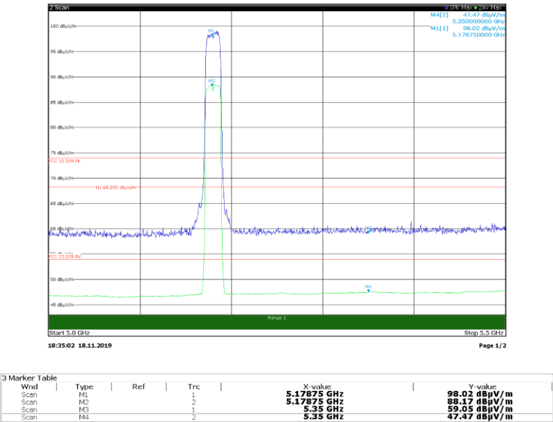
Band edge bands, Tx on 5180 MHz, 802.11 Nht20 horizontal
