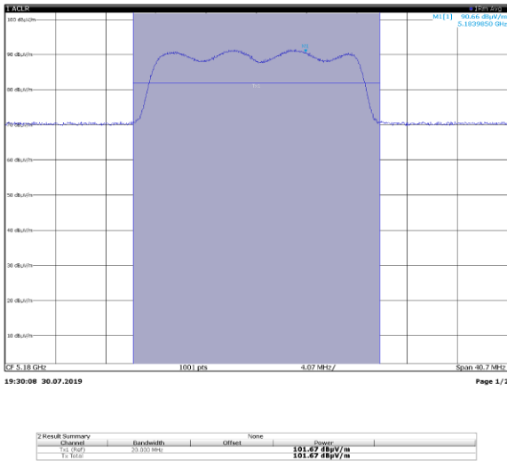
PSD on 802.11a Sample plot, vertical
