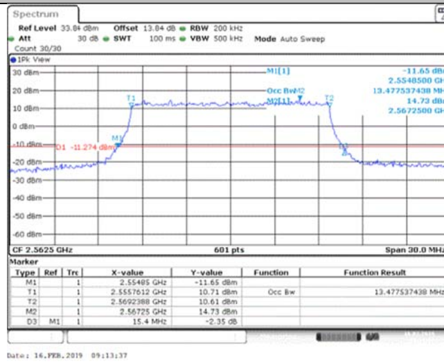
Band41_15MHz_16QAM_40740_75RB#0
