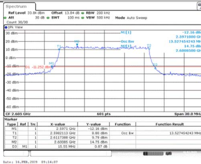
Band41_15MHz_16QAM_40740_75RB#0
