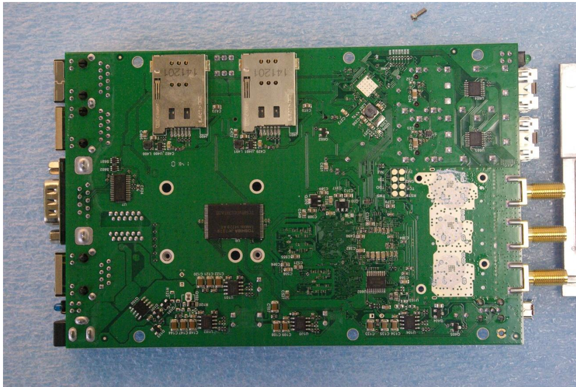
Back side of module with heat sink removed
