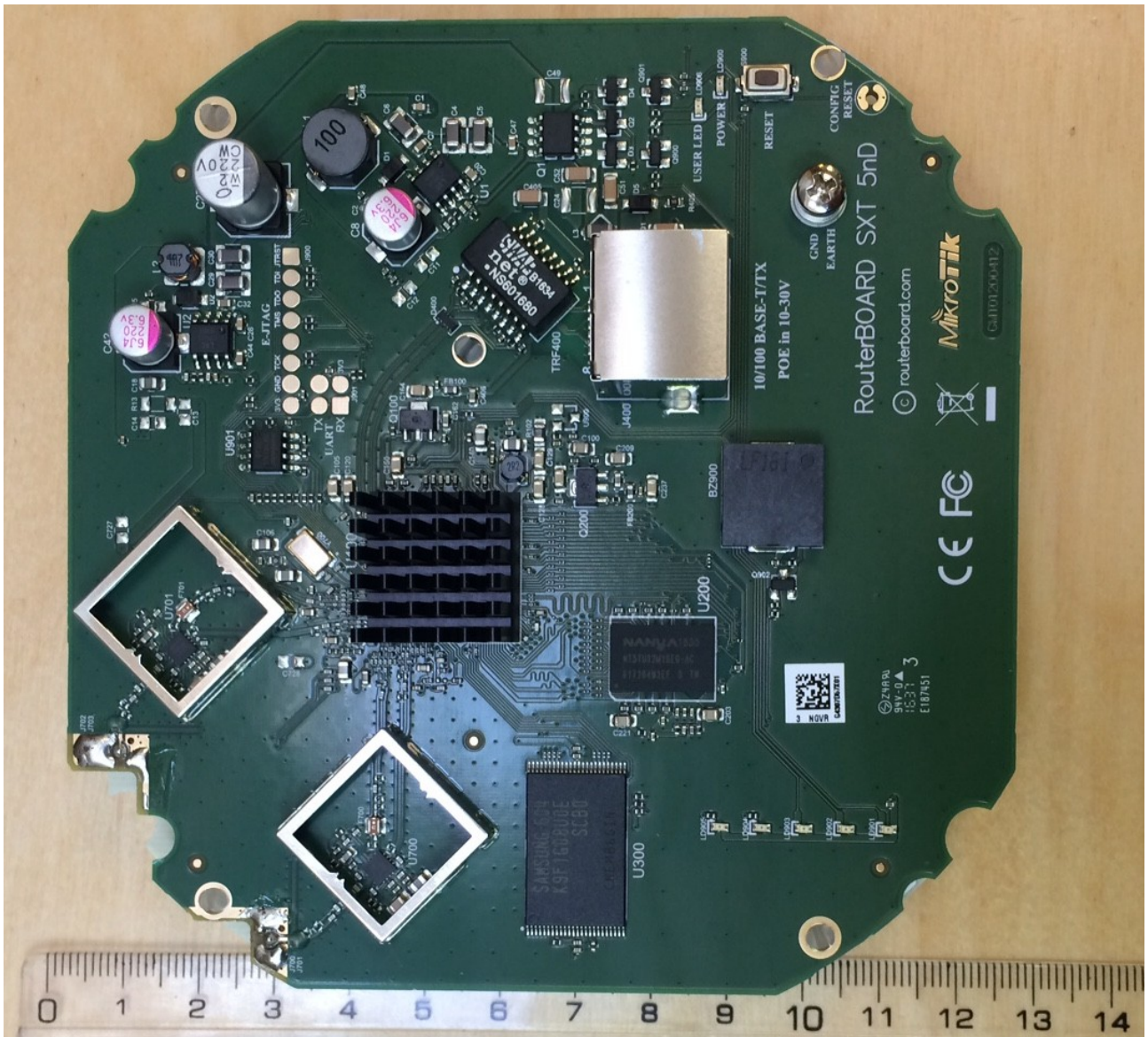
Internal Photos of EUT
