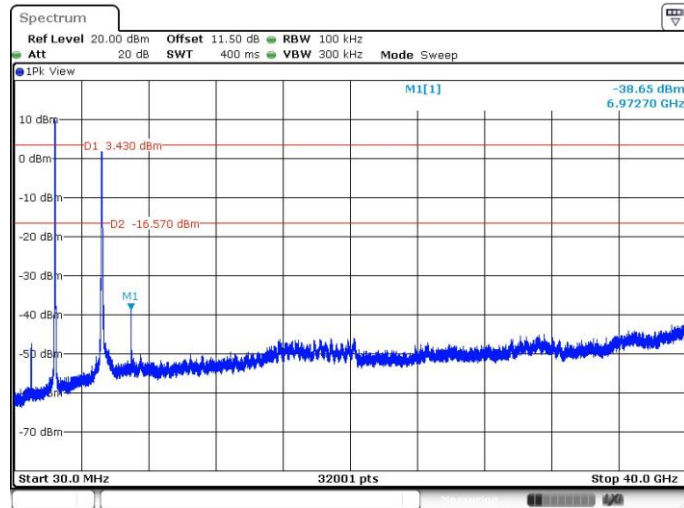
Conducted Emission Plots of Antenna port chain 0
