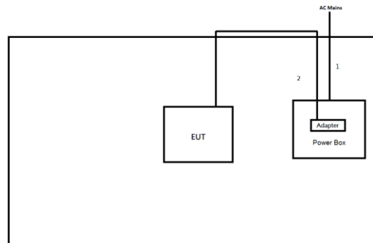
Test Setup Diagram - Radiated Test (Non-Beamforming)
