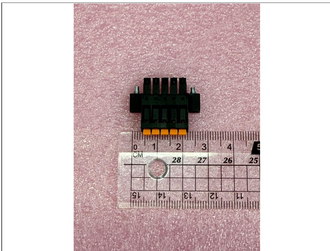
Digital I/O Connector (Brand: PHOENIX, Model: 1688289)
