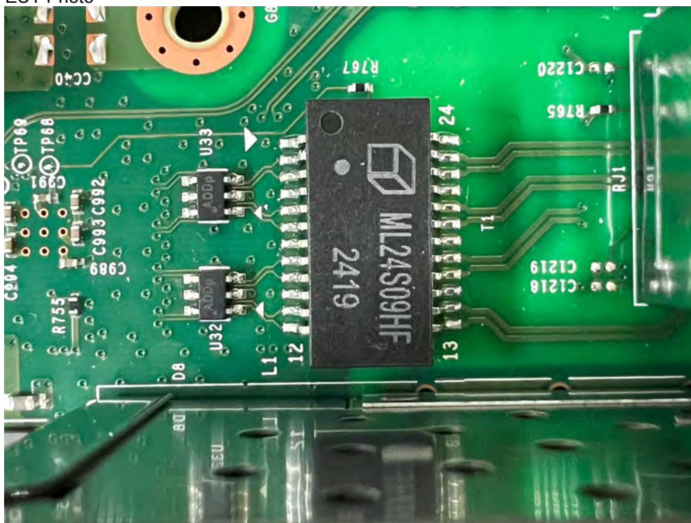
(68) EUT Photo
