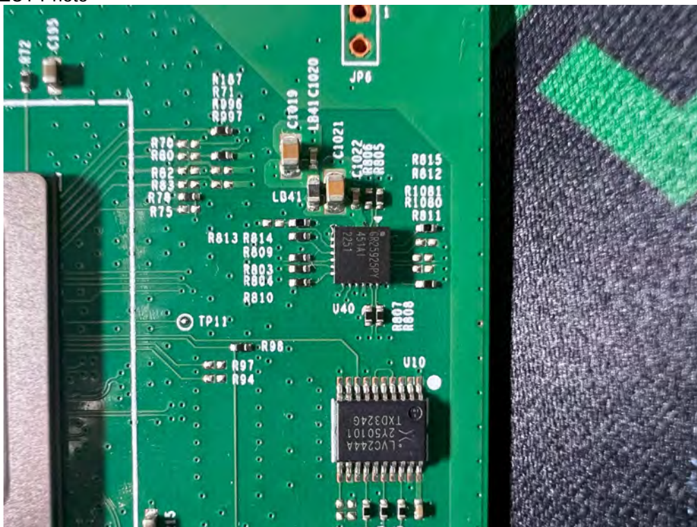
(68) EUT Photo
