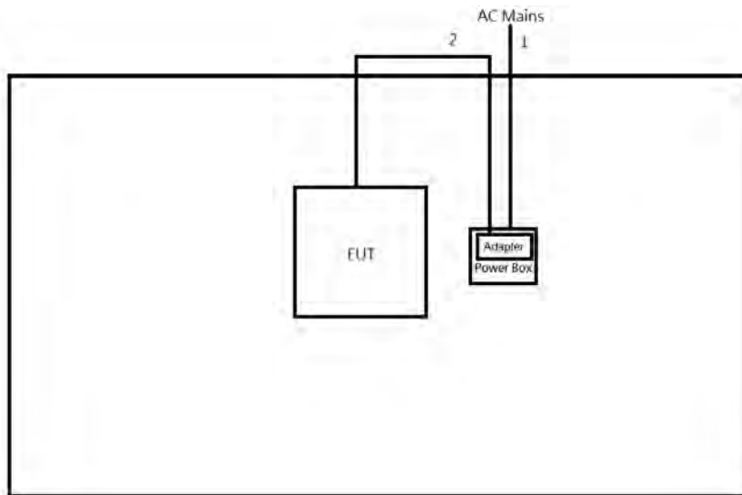
Test Setup Diagram – Radiated Test (Adapter Mode)
