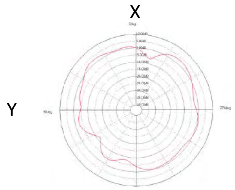
theta 90° plane
