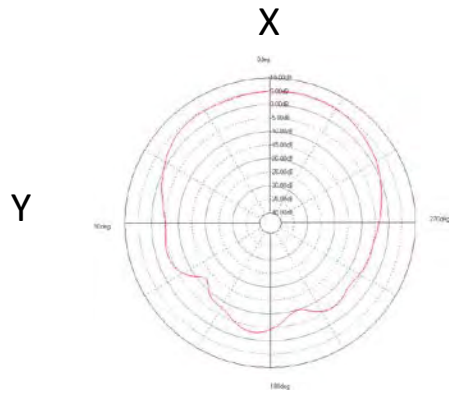
theta 60° plane
