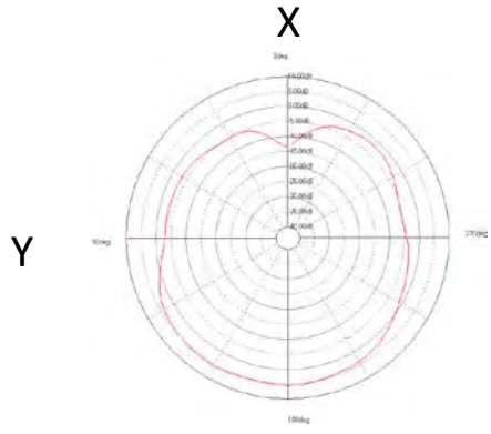
theta 60° plane
