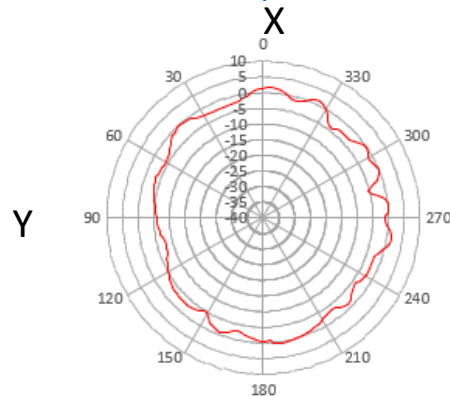
theta 90° plane
