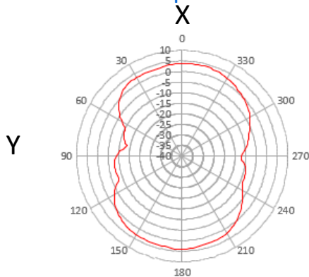
theta 90° plane
