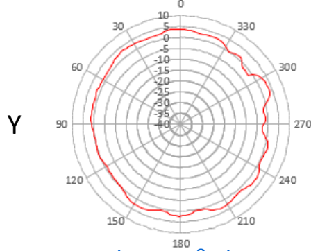
theta 60° plane
