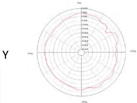
theta 60° plane
