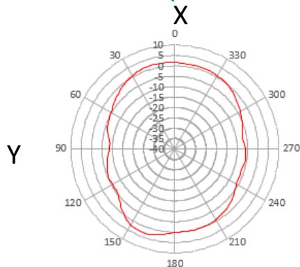
theta 90° plane
