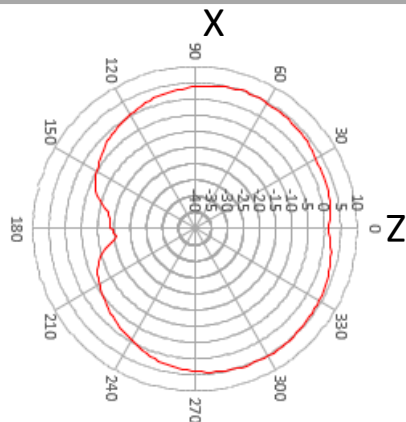
X-Z plane
