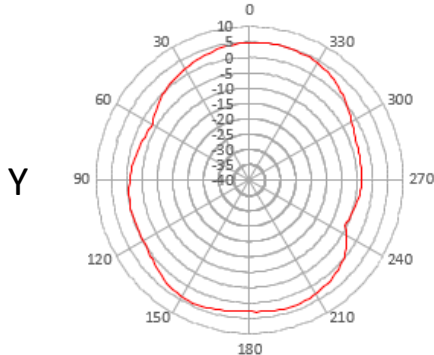
theta 60° plane
