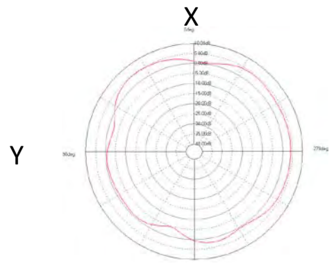
theta 60° plane
