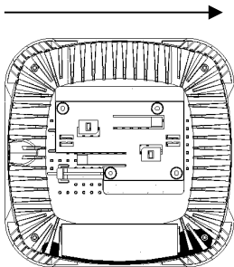
Ceiling Bracket Install Slide Direction
