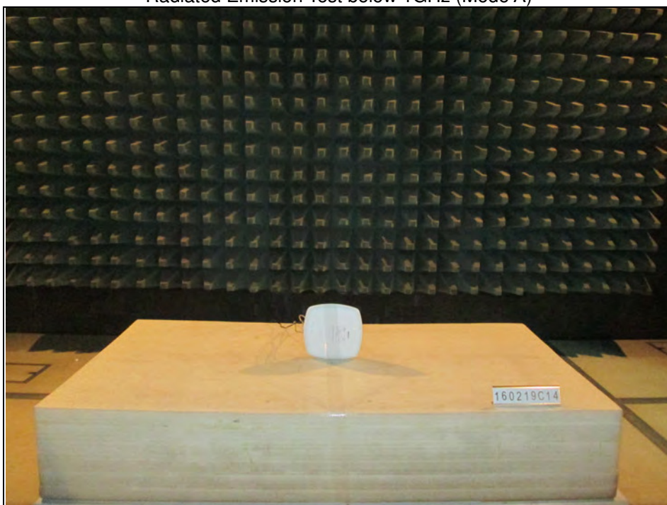
Radiated Emission Test below 1GHz (Mode A)
