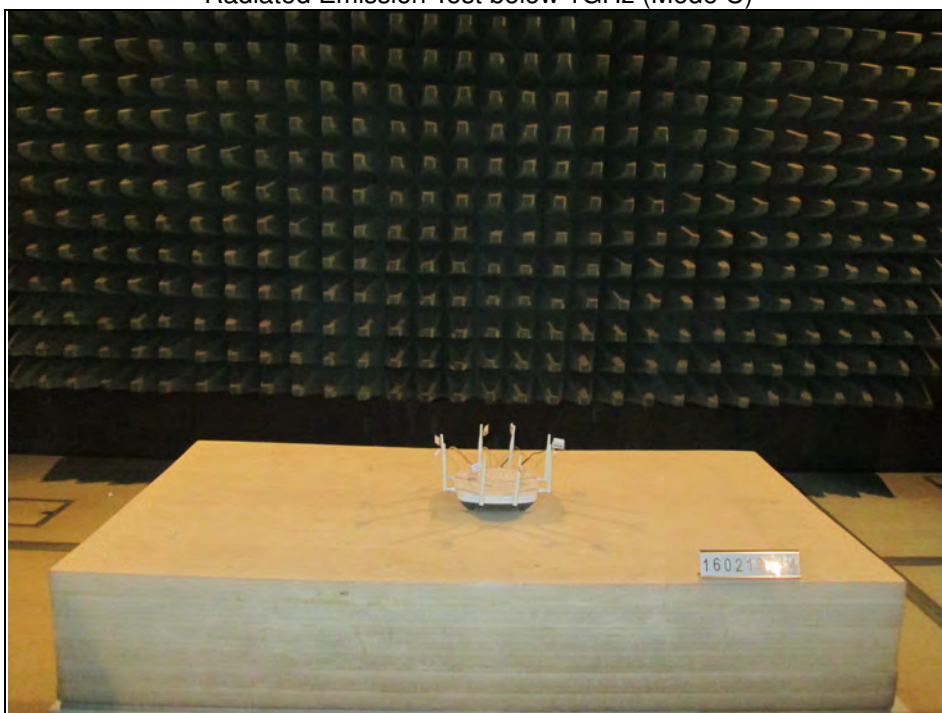
Radiated Emission Test below 1GHz (Mode C)
