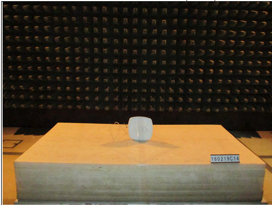
Radiated Emission Test below 1GHz (Mode B)
