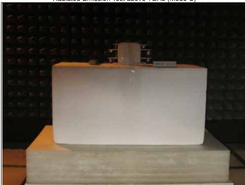
Radiated Emission Test above 1GHz (Mode C)
