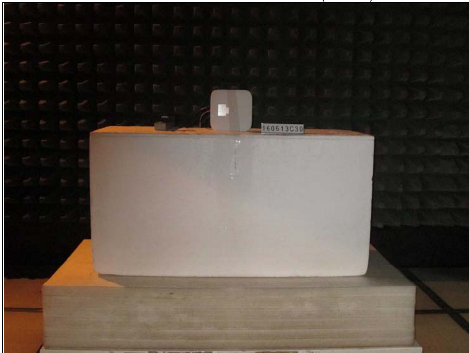
Radiated Emission Test above 1GHz (Mode A)
