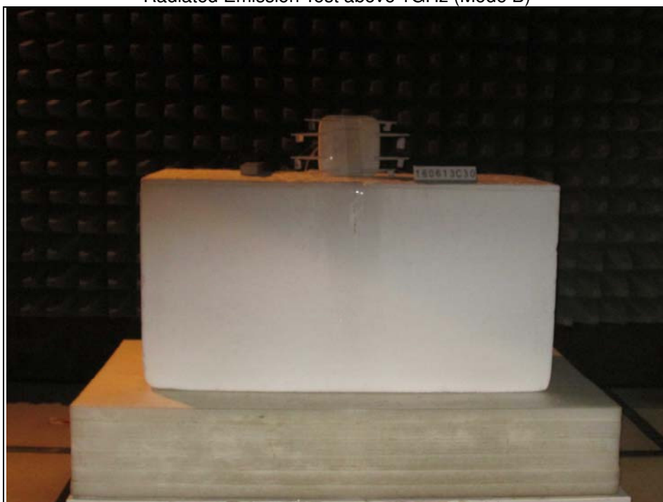
Radiated Emission Test above 1GHz (Mode B)
