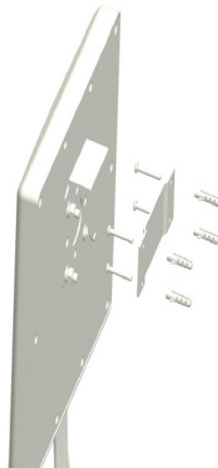
Wall Mounting
