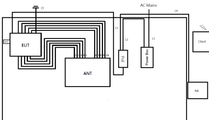
Test Setup Diagram - Radiated Test (Beamforming)
