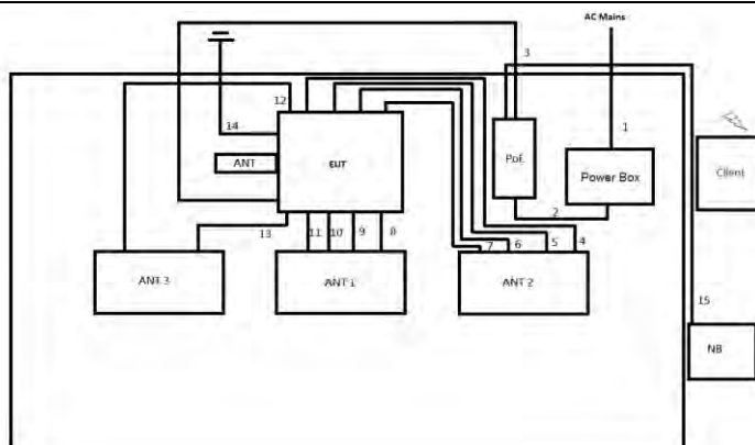
Test Setup Diagram - Radiated Test – Beamforming_Radio 1
