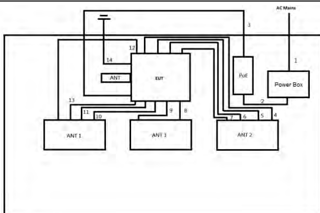
Test Setup Diagram - Radiated Test – Non-Beamforming_Radio 3
