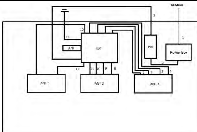
Test Setup Diagram - Radiated Test – Non-Beamforming_Radio 2
