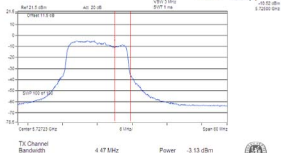
Chain 1/CH 144 (For U-NII-3)
