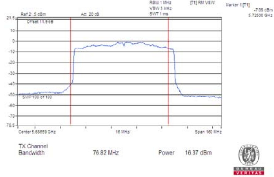
Chain 3/CH 138 (For U-NII-2C)
