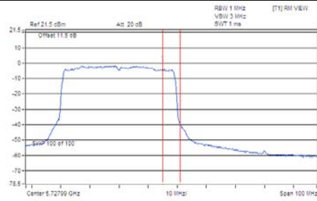
Chain 3/CH 142 (For U-NII-3)
