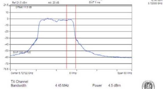
Chain 3/CH 144 (For U-NII-3)
