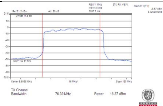
Chain 1/CH 138 (For U-NII-2C)
