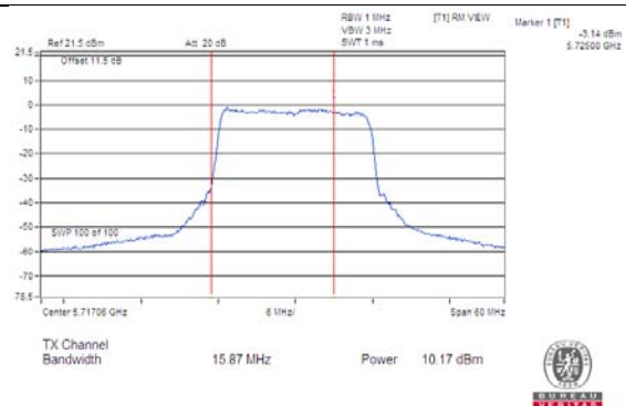
Chain 1/CH 144 (For U-NII-2C)
