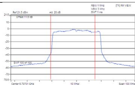
Chain 0/CH 142 (For U-NII-2C)
