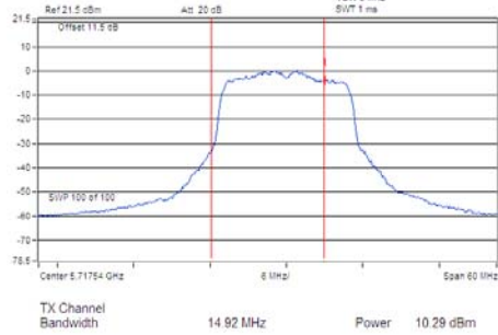
Chain 2/CH 144 (For U-NII-2C)
