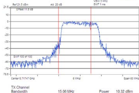
Chain 1/CH 144 (For U-NII-2C)
