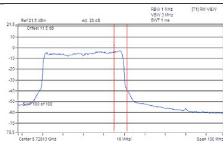
Chain 0/CH 142 (For U-NII-3)
