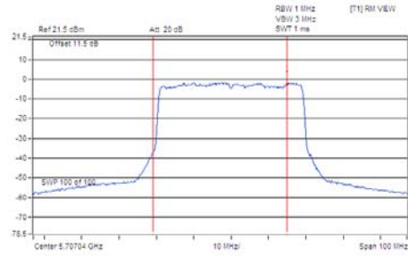
Chain 2/CH 142 (For U-NII-2C)
