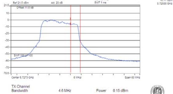
Chain 2/CH 144 (For U-NII-3)
