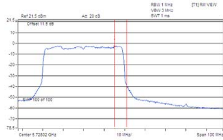
Chain 2/CH 142 (For U-NII-3)
