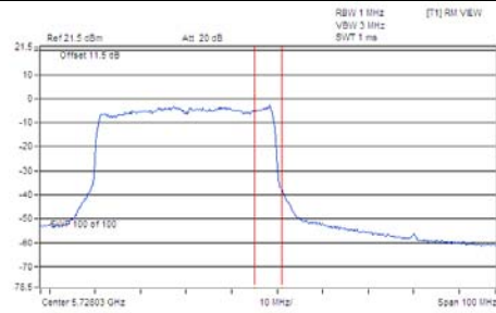
Chain 1/CH 142 (For U-NII-3)
