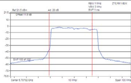
Chain 1/CH 142 (For U-NII-2C)
