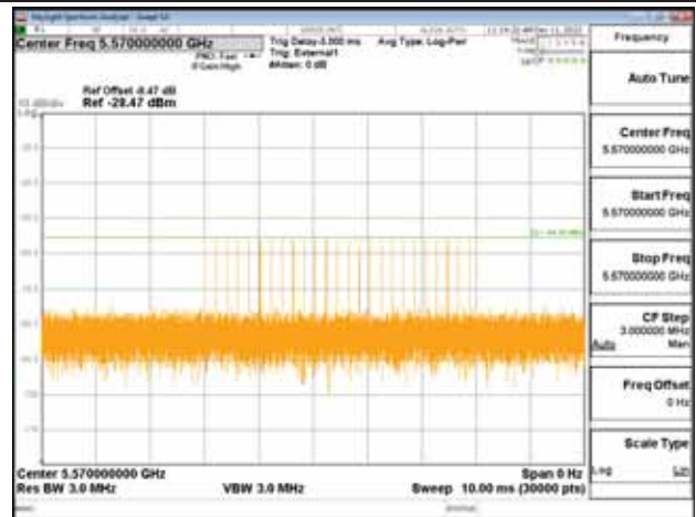
Radar Type 2
