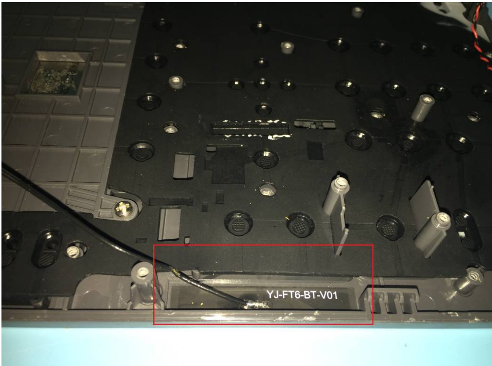
BT Antenna
