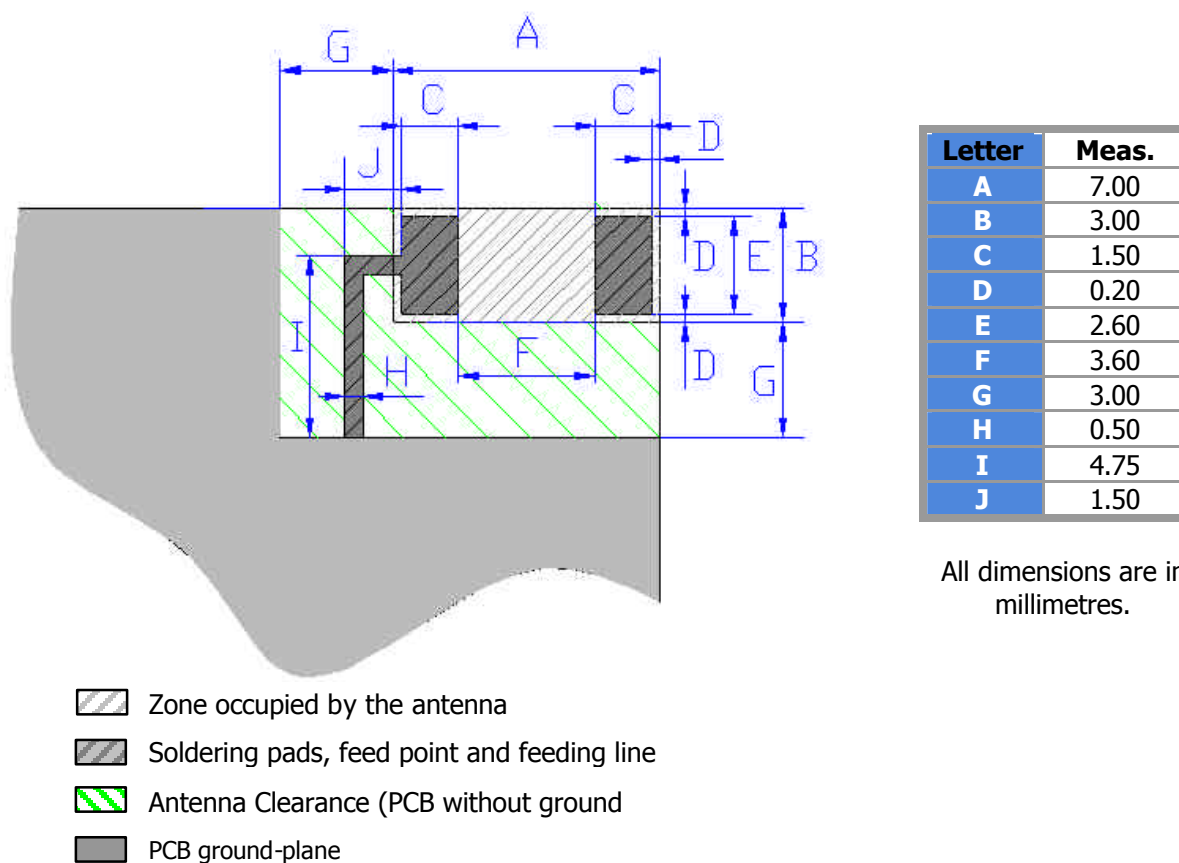
Figure 2. Antenna Footprint
