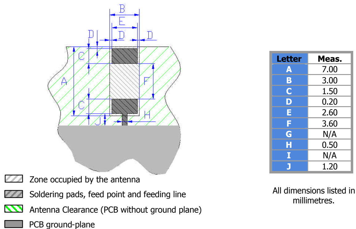
Figure 7. Antenna Footprint
