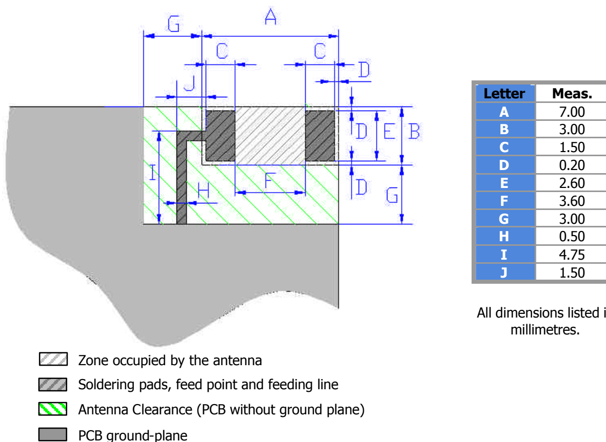
Figure 4. Antenna Footprint
