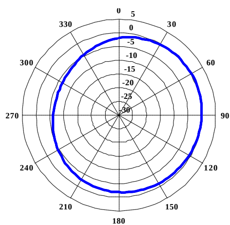
Azimuth Cut
