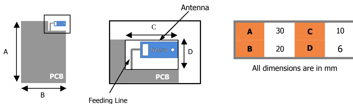
Figure 3. PCB Dimensions and Clearance Dimensions.
