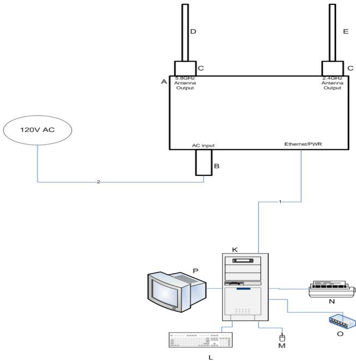
Figure 1. Block Diagram of Test Configuration, AC Mode
