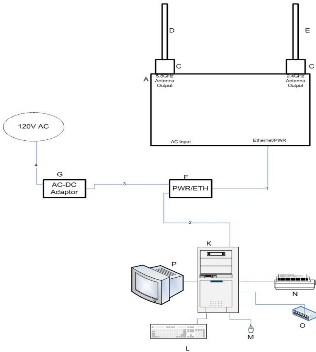
Figure 2. Block Diagram of Test Configuration (Conducted Measurement)
