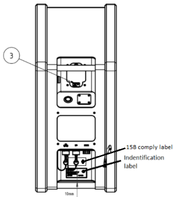
Flux systembox back side
