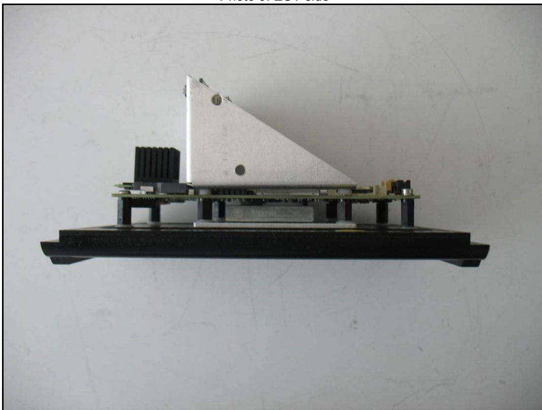
Photo 9: EUT side
