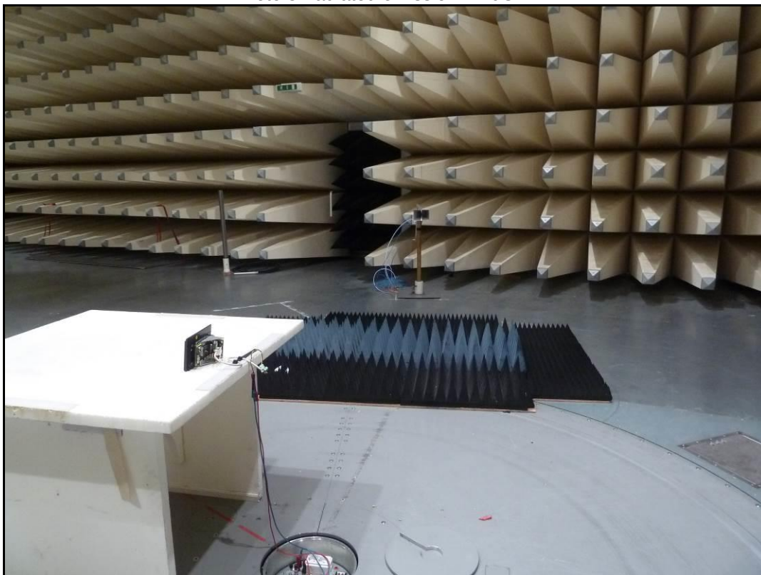
Photo 4: radiated emission > 10GHz
