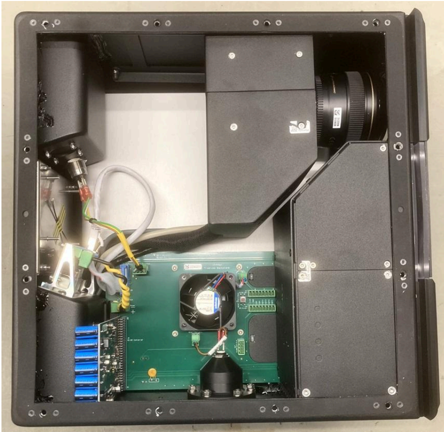
Figure 1: Right side of T-Series RT4.1 (cover plate removed)
