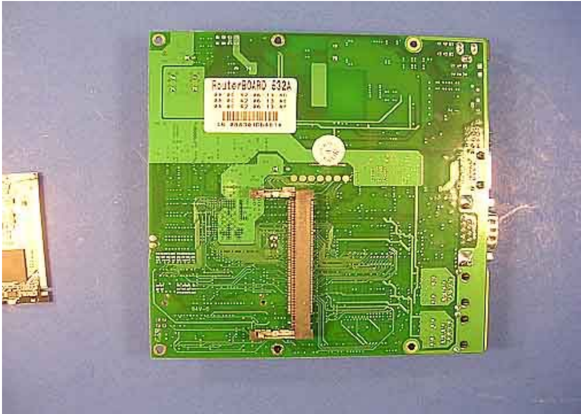
2407M Main Board Bottom
