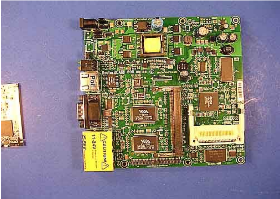
2407M Main Board Top
