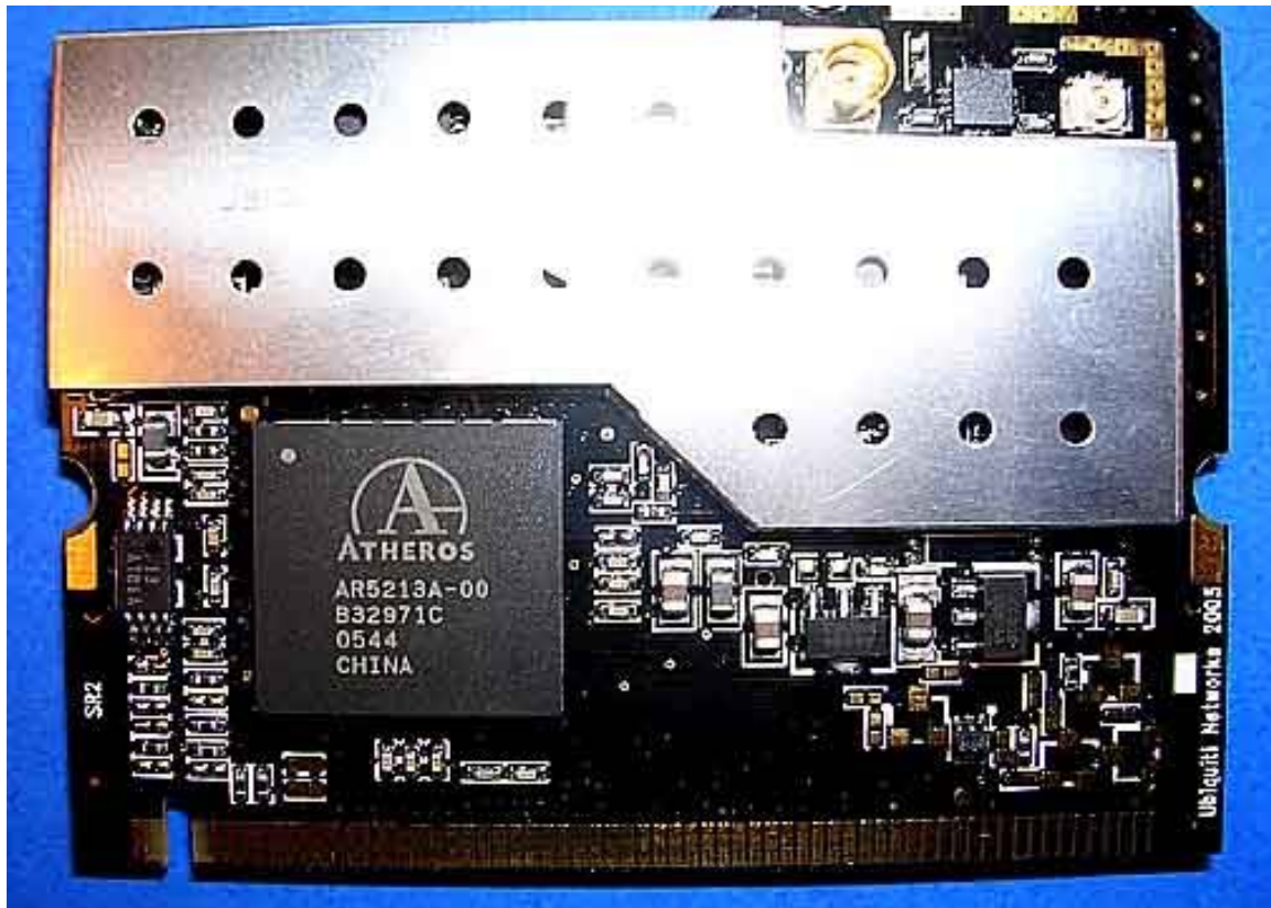
24150 Transmitter Board Top
