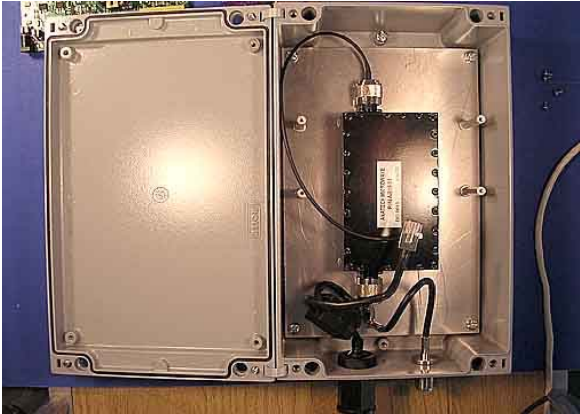
24150 Filter on Ground Plane
