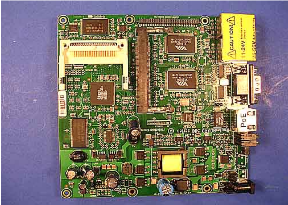
24150 Main Board Top
