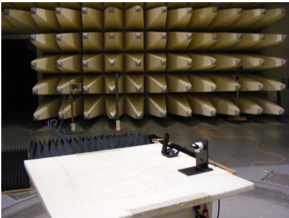
Photo 2: Radiated Emission
