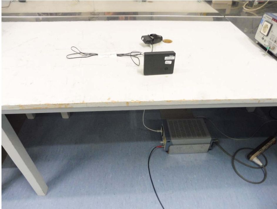
Photo 3: Conducted Emission
