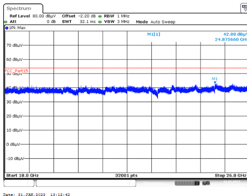
Plot 4: 18 GHz to 26 GHz, TX mode, valid for all channels, vertical & horizontal polarization
