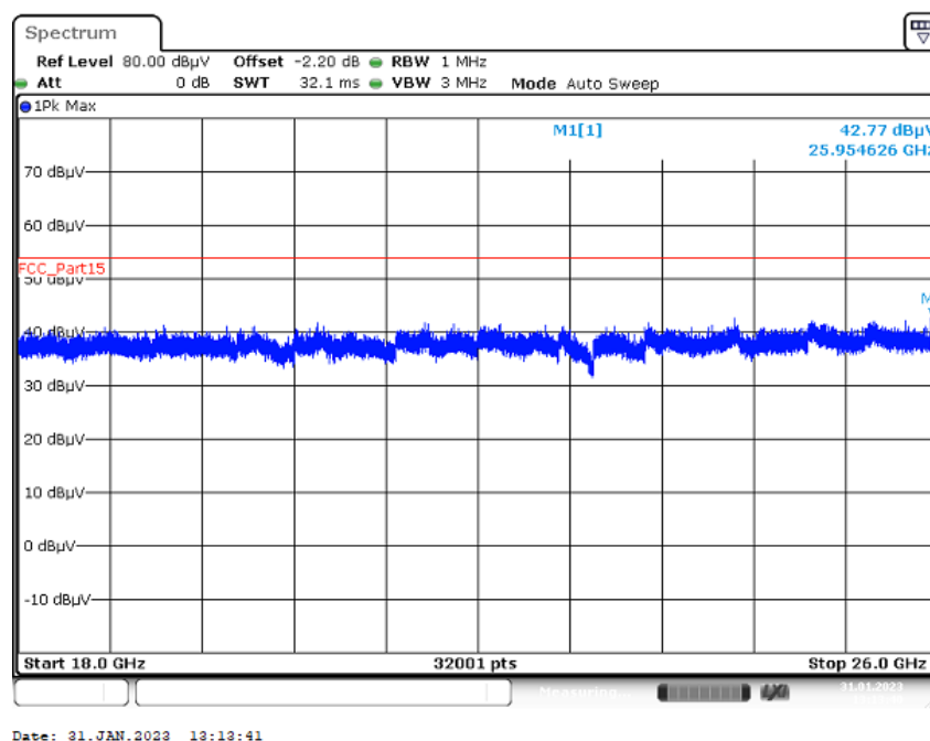
Plot 4: 18 GHz to 26 GHz, TX mode, valid for all channels, vertical & horizontal polarization, 1 Msp/s
