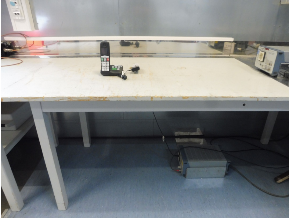
Photo 3: Conducted Emission
