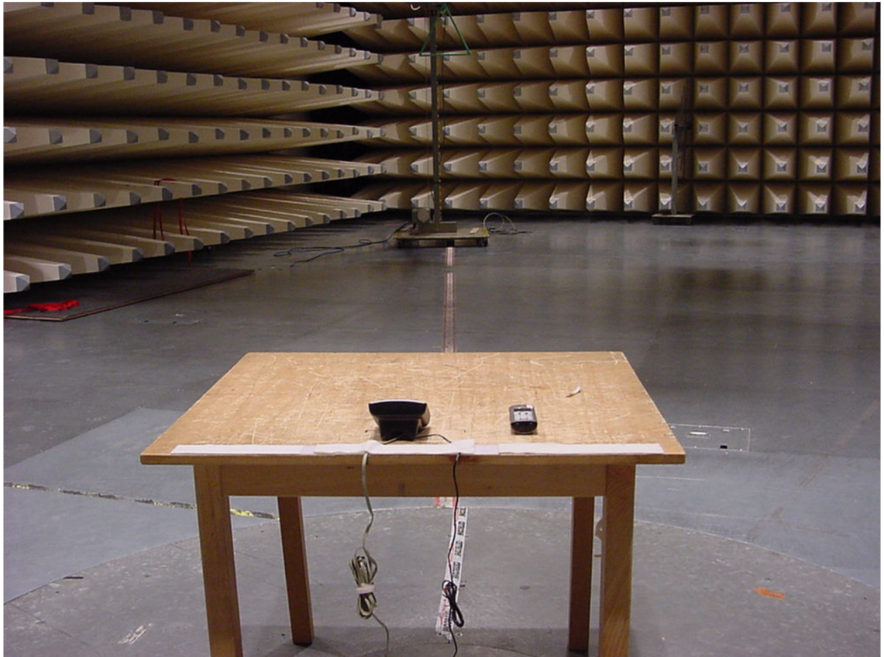
Photo 1: Radiated Emissions
