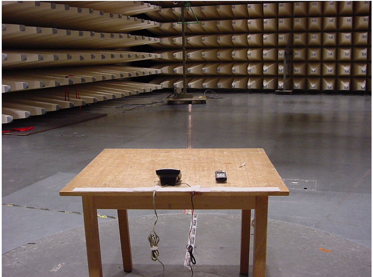
Photo 1: Radiated Emissions
