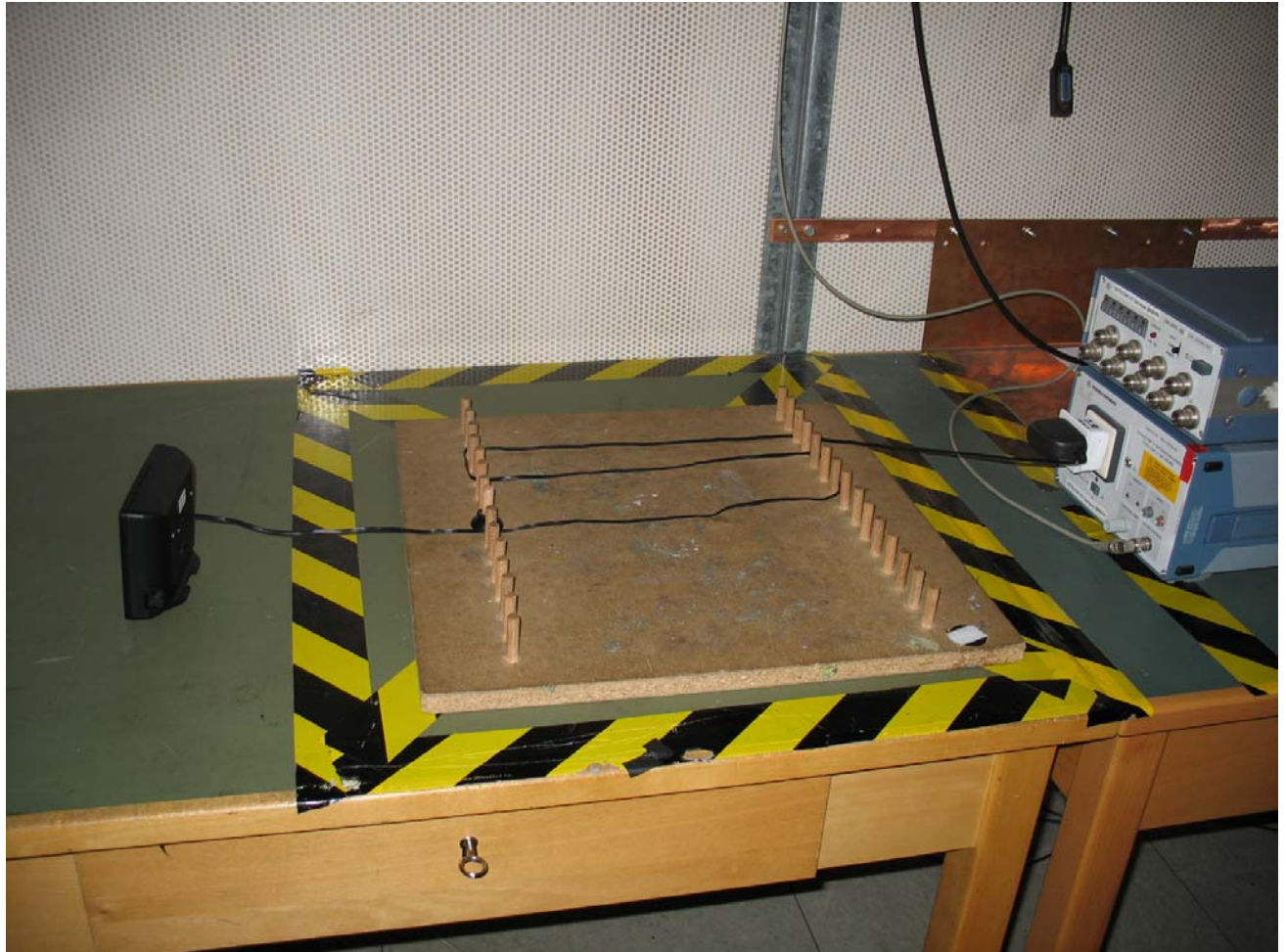
Photo 3: Conducted Emissions
