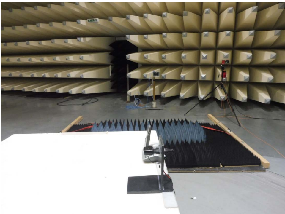
Photo 2: Radiated Emission
