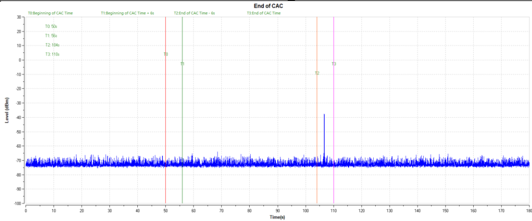
11AX20SISO_5500
