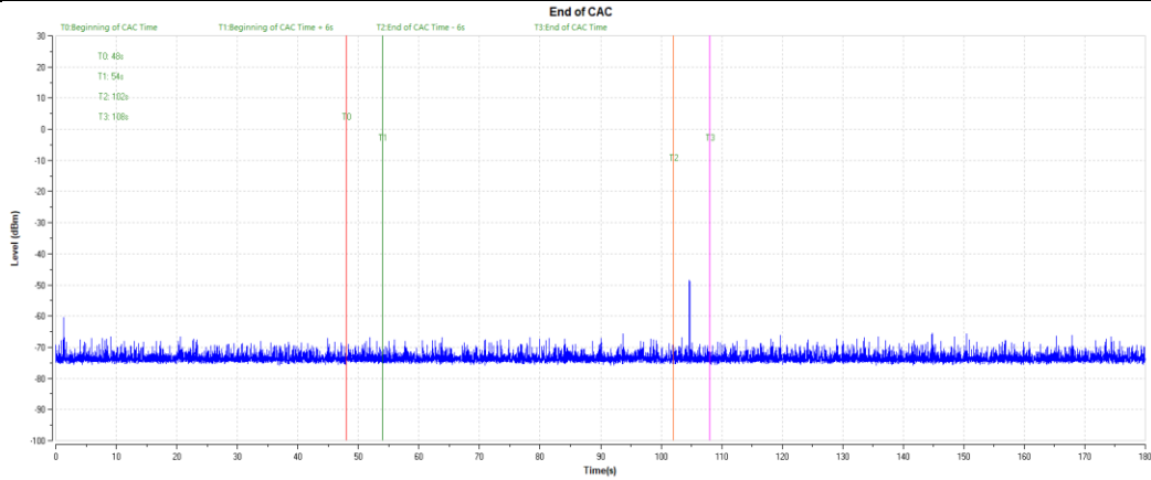
11AX20SISO_5260
