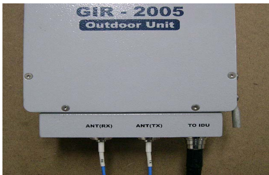
Figure 3-5 ODU connected to IDU & Internal Antenna using cables
