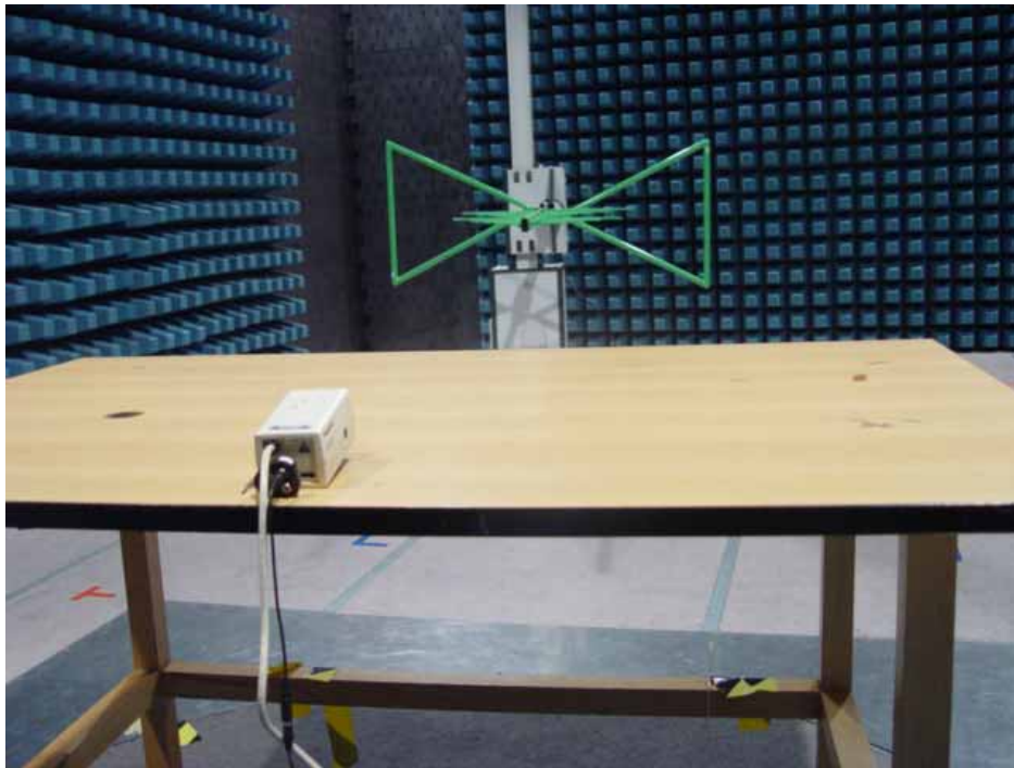
Photo 3 Radiated Emission Test
